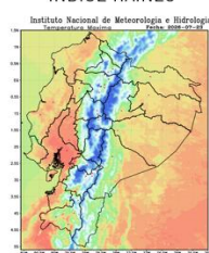
INDICE HAINES
